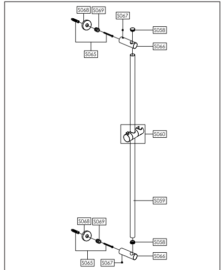
Explosive drawing
