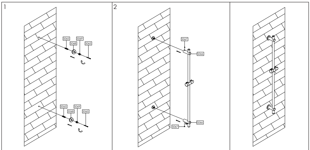
Installation Steps
